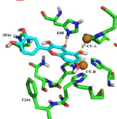
Quercetin and tyrosinase interaction
